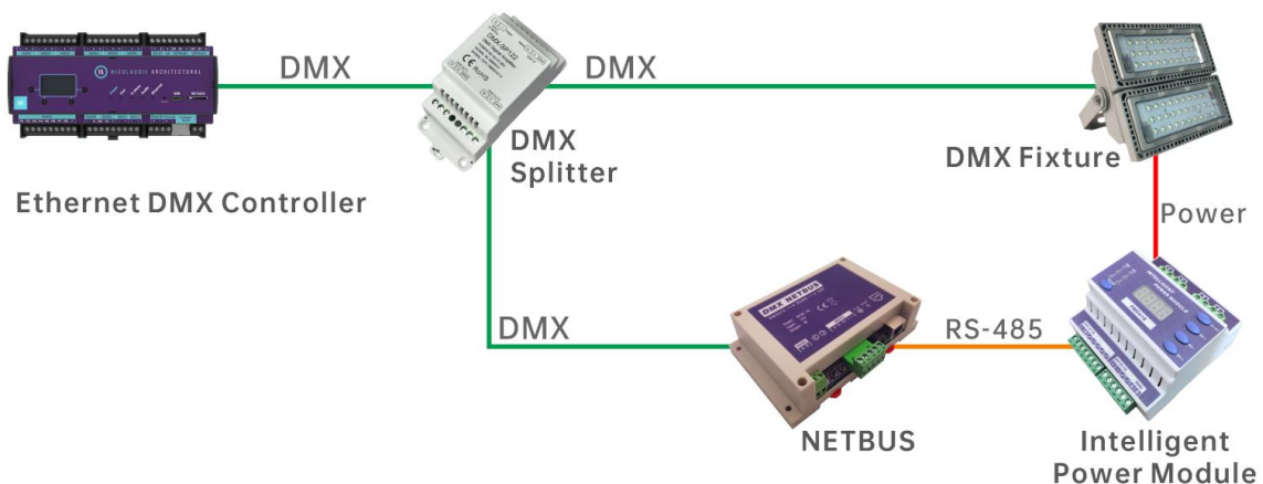
DMX NETBUS Wire Diagram (DMX & Power Control)
